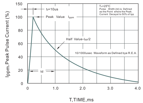
Fig.2 Pulse Waveform
