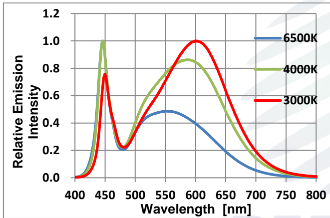
Typical spectrum distribution 典型光谱分布
