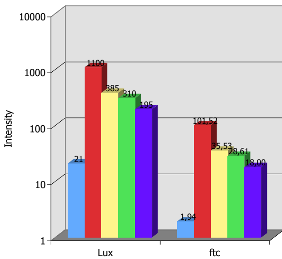
Intensity to 1 Meter
