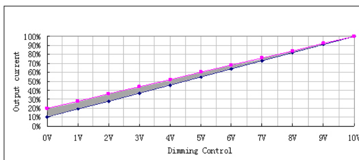
Implementation 2: DC input
